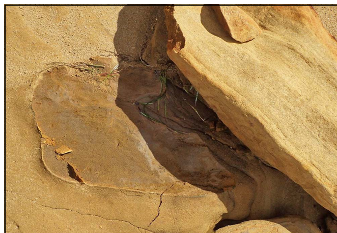
Fig. 5. When I prised the second cobble loose, it was clear its base had been abraded flat, and the cobble itself had wiggled itself several millimetres into the host sandstone. The darker colour is where the cobble had been sitting. Photo width 40 cm.
